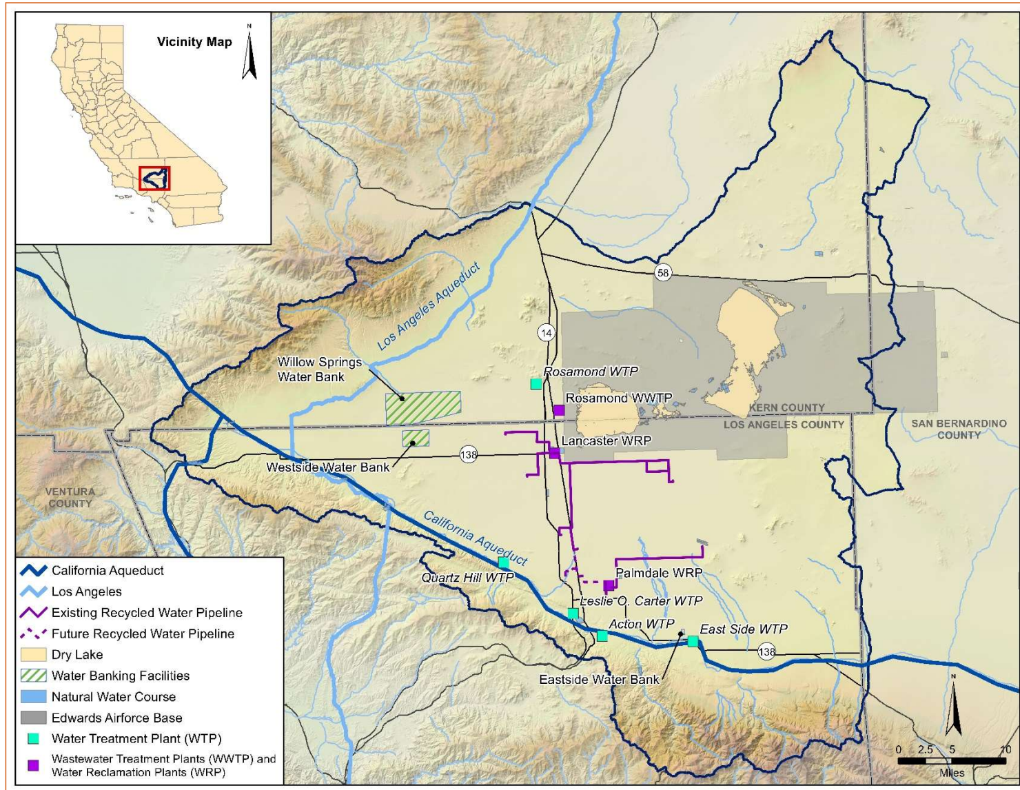
Figure 3-2: Major Infrastructure
